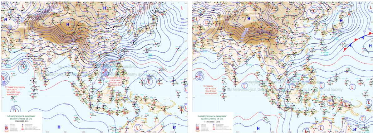
Figure 1: Summary of weather condition over the LMB from 5 and 9 Dec 2019
